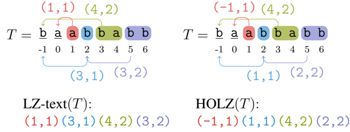
Figure 2: LZ factorization of T = abbabb with its LZ-text ( left ) and HOLZ encoding ( right ). Since the encodings only differ in the values of their offsets, they are equal in length.
